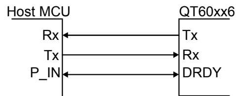
Figure 3-5 UART Connections
