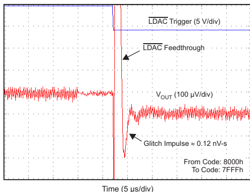
Figure 38. Glitch Impulse Falling Edge, 1-LSB Step
