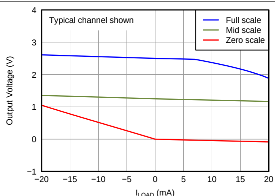
Figure 74. DAC Output Voltage vs Load Current
