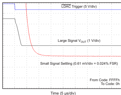
Figure 76. Full-Scale Settling Time: Falling Edge
