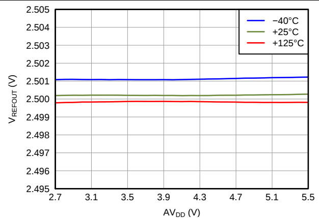
Figure 7. Internal Reference Voltage vs Supply Voltage
