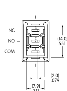
Single Pole
