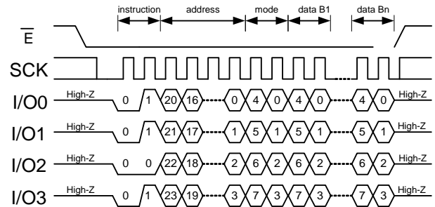
F_READ in QPI Mode
