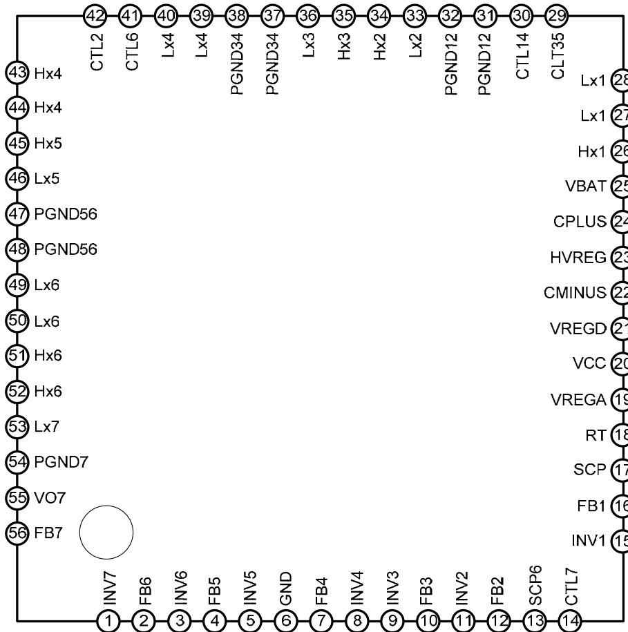
Fig. 2 Pin Assignments
