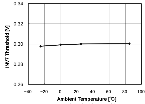
Fig. 17 CH7 ErrorAmp. INV threshold vs ambient temperature
