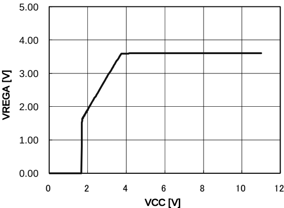
Fig. 12 VREGA vs supply voltage
