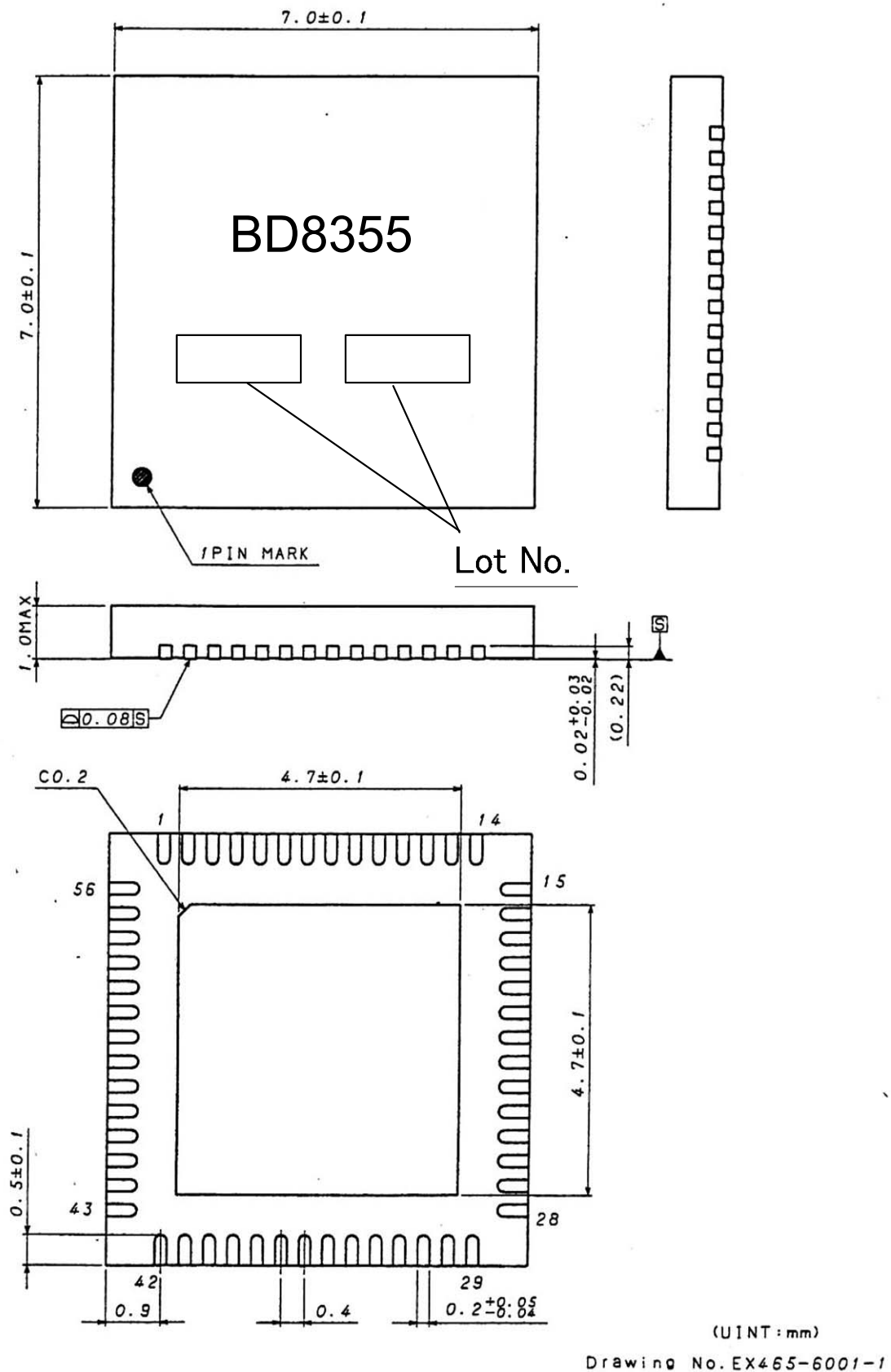
Fig. 1 Package dimension
