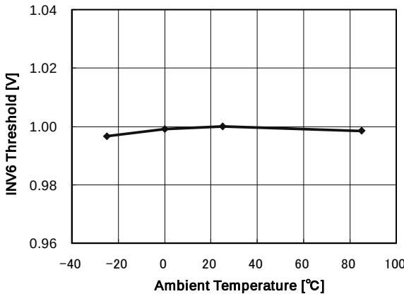
Fig. 16 CH6 ErrorAmp. INV threshold vs ambient temperature
