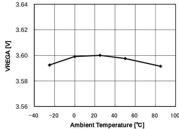
Fig. 13 VREGA vs ambient temperature
