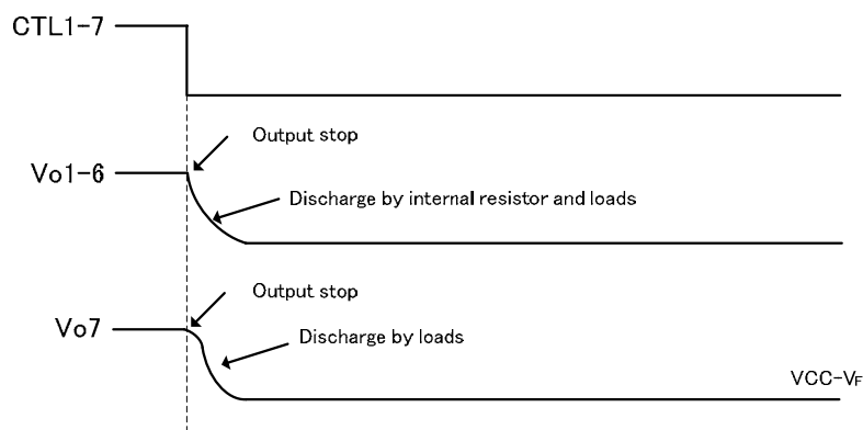
Fig. 6 stop sequence
