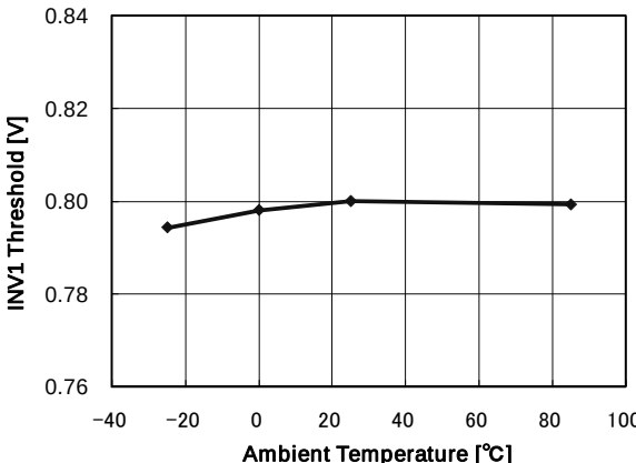
Fig. 14 CH1 ErrorAmp. INV threshold vs ambient temperature
