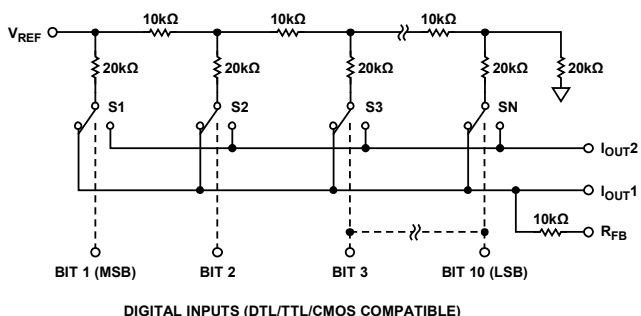
Figure 7. Functional Diagram
