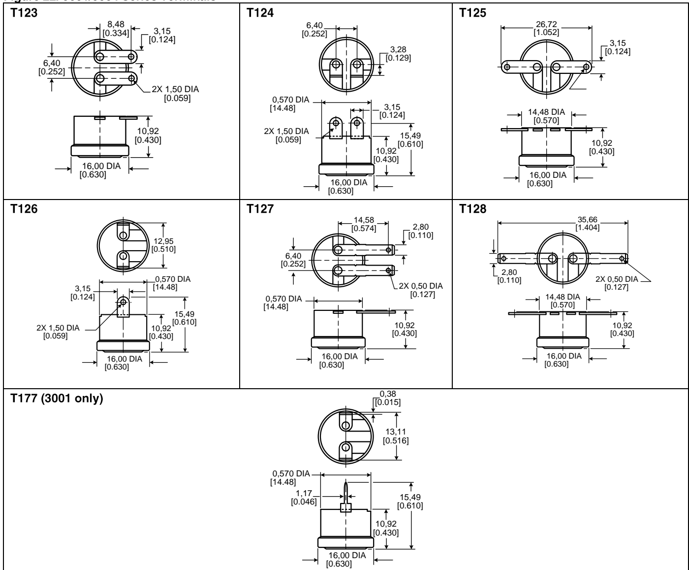
Figure 22. 3001/3004 Series Terminals
