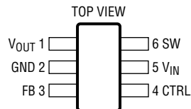
S6 PACKAGE 6-LEAD PLASTIC TSOT-23
