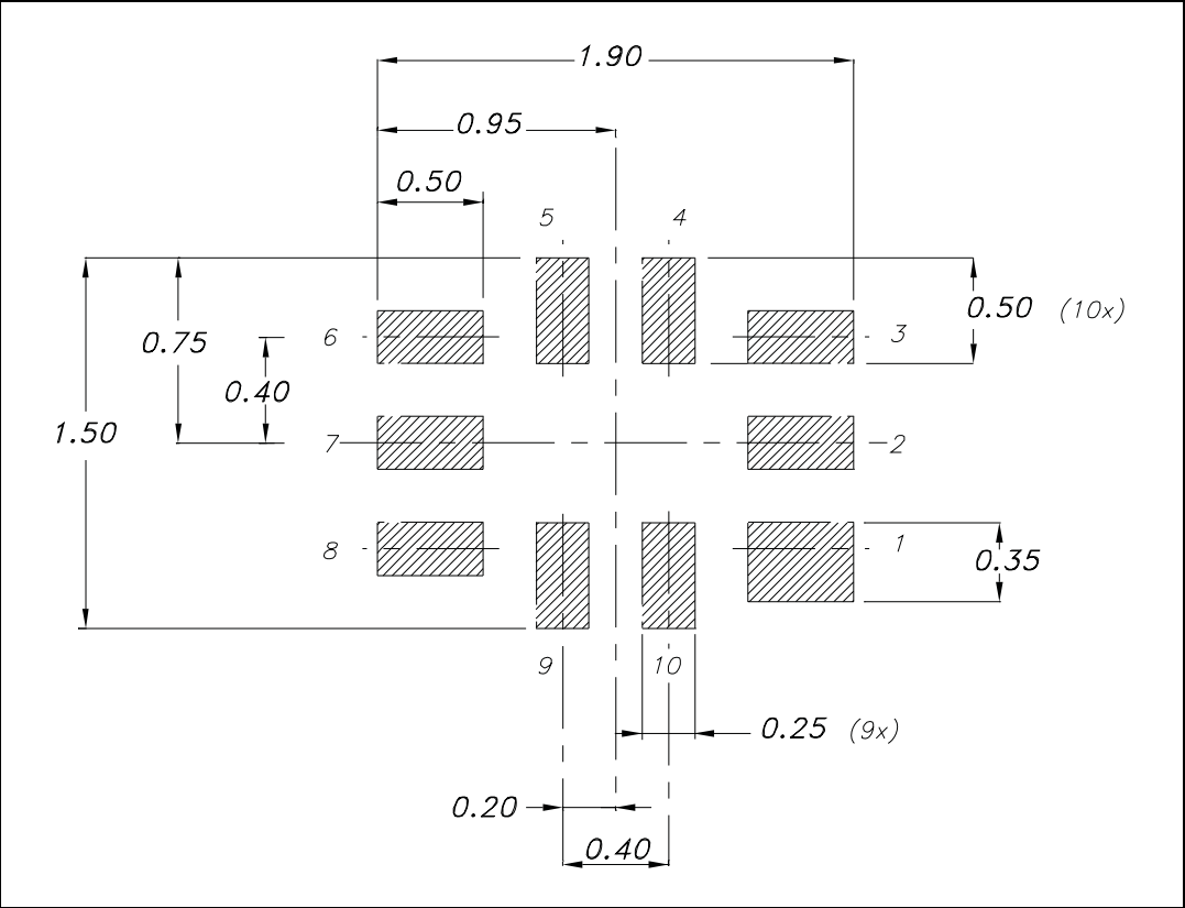
Figure 8. QFN10L (1.8 mm x 1.4 mm) footprint recommendation
