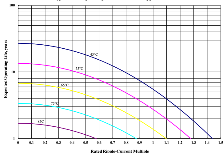
Type THAS Operating Life in Years vs Ripple Current
