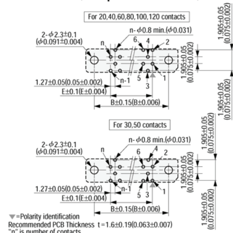
Printed Circuit Board Layout (Component Side View)
