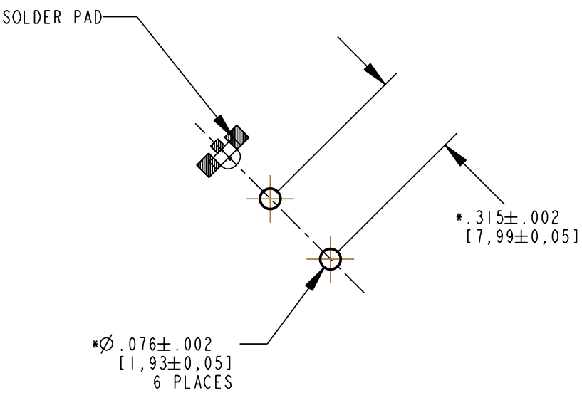
RECOMMENDED HOLE PATTERN LAYOUT FOR 1 POSITION STRAIGHT LIGHTPIPE 515-1154F
