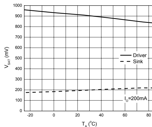
Figure 11. V SAT vs. Ambient Temperature
