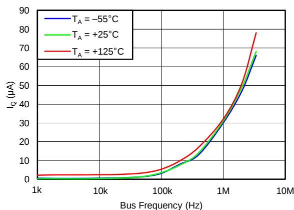
Figure 4. QUIESCENT CURRENT vs BUS FREQUENCY
