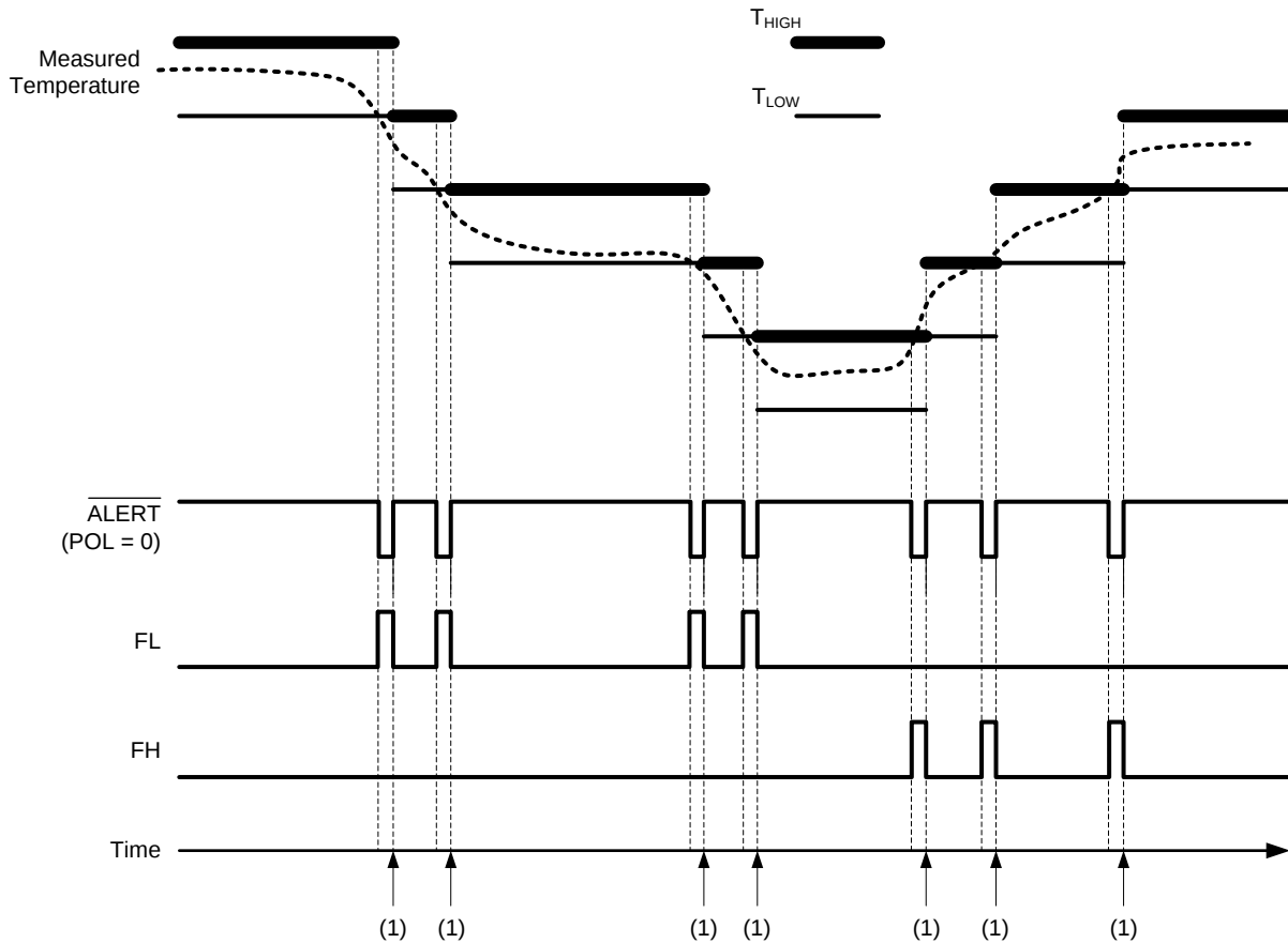
Figure 10. Interrupt Mode
