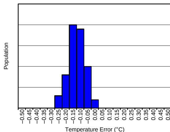
Figure 6. TEMPERATURE ERROR AT +25^\circ\text{C}
