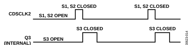
Figure 13. SHA Mode Internal Switch Timing
