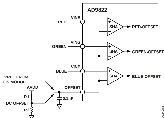
Figure 14. SHA Mode Used with External DC Offset
