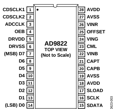
Figure 2. Pin Configuration
