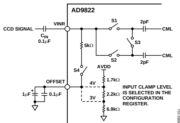
Figure 10. CDS Mode Input Configuration (All Three Channels are Identical)
