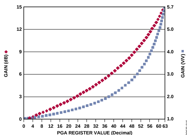
Figure 15. PGA Gain Transfer Function
