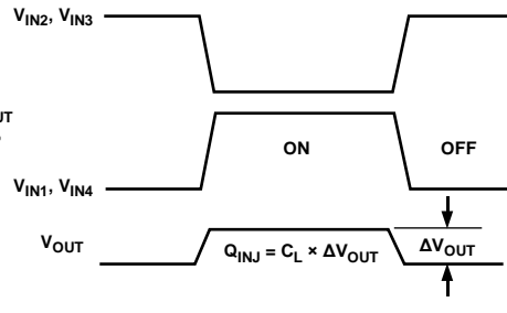
Figure 19. Charge Injection
