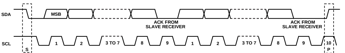
Figure 53. Acknowledge Bit
