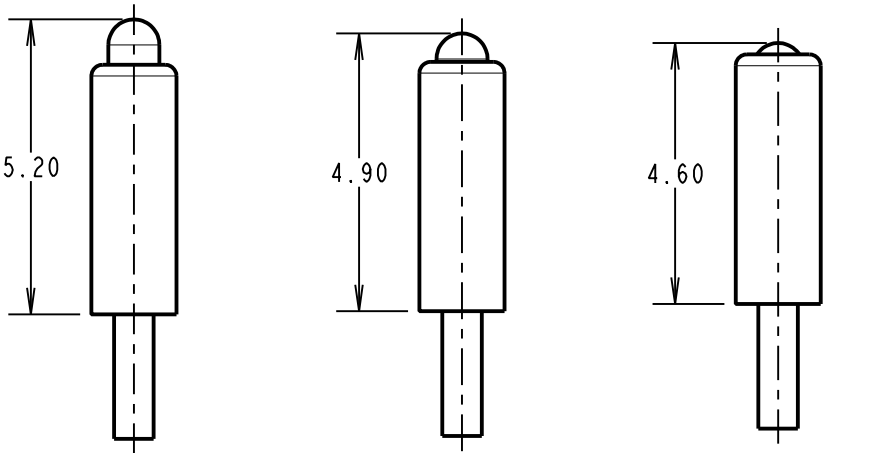
MINIMUM WORKING HEIGHT/MAX ALLOWED TRAVEL
