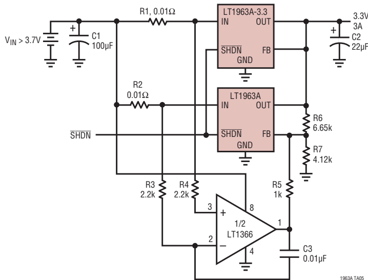
Paralleling of Regulators for Higher Output Current
