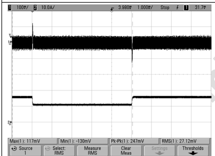
Step Load Transient Response@25°C (Vin = 110V, Vout = nom., Iout = 75-50-75% of full load, Cloud = 0µF, ScopeBW = 20MHz)
