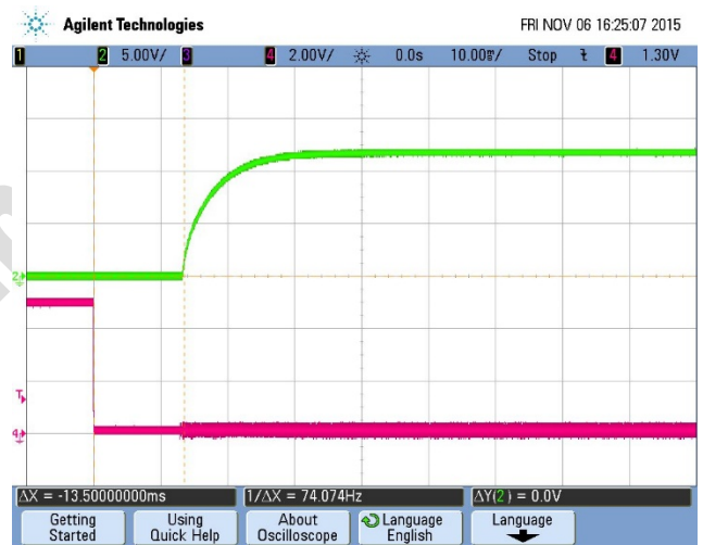
Turn-on transient at full load current (10 mS/div, Top Trace: Vout, 5V/div; Bottom Trace: ON/OFF, 2V/div)
