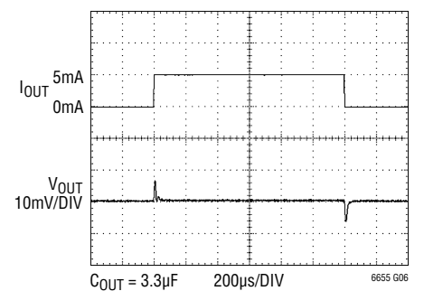
1.25V Sinking Current with a 3.3μF Output Capacitor
