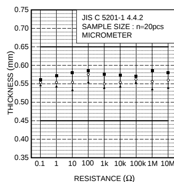
Fig.4 Dimensions (thickness)
