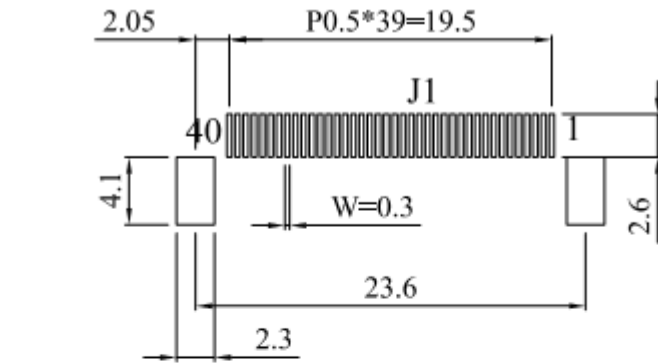
DETAIL J1 SCALE 2/1
