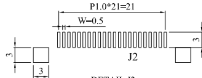
DETAIL J2 SCALE 2/1
