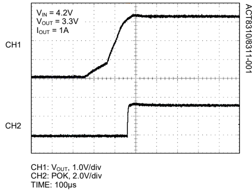
Startup Waveform
