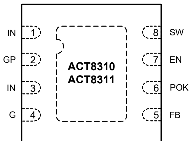
TDFN33-8
