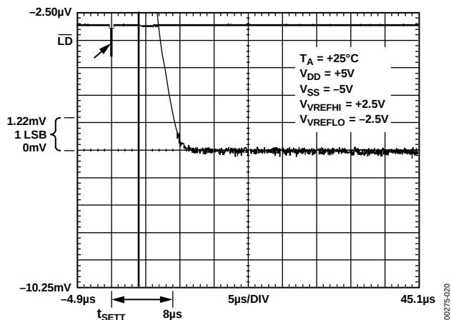
Figure 19. Positive Settling Time ( \pm 5\text{ V} )
