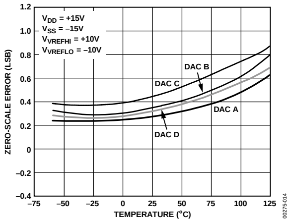
Figure 13. Zero-Scale Error vs. Temperature
