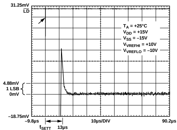
Figure 21. Positive Settling Time ( \pm 15\text{ V} )
