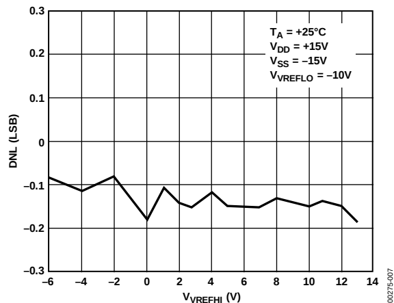
Figure 6. DNL vs. V_{REFHI} ( \pm 15\text{ V} )
