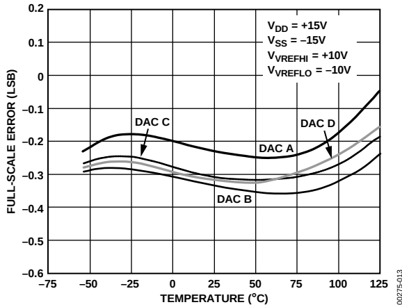
Figure 12. Full-Scale Error vs. Temperature
