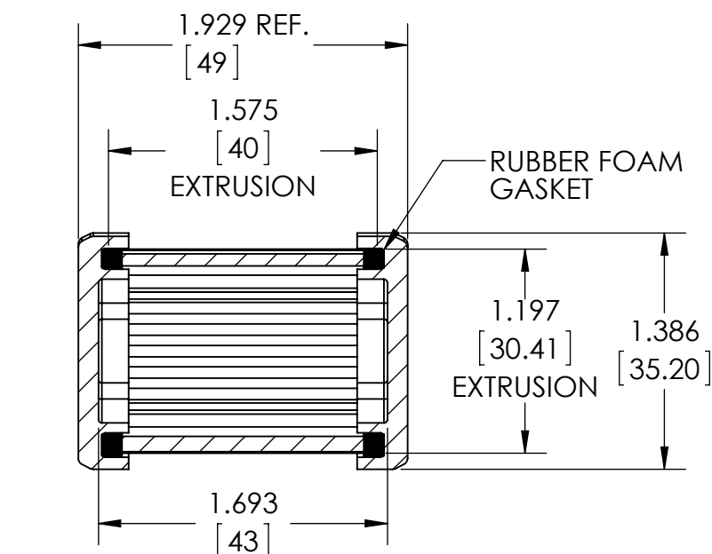
SECTION A-A DIMENSIONS MAY VARY DEPENDING ON THE COMPRESSION OF THE GASKETS
