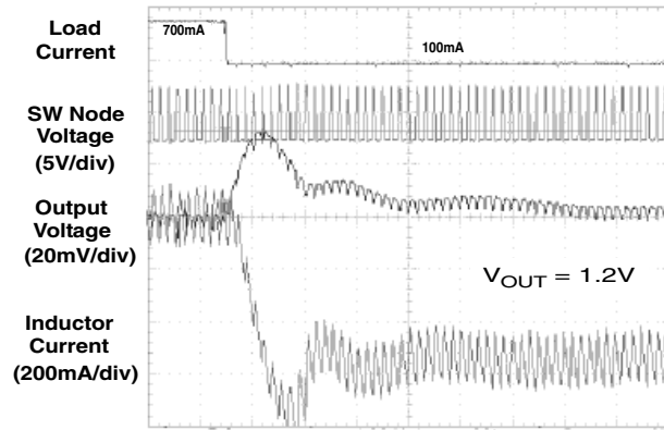
Transient Response
