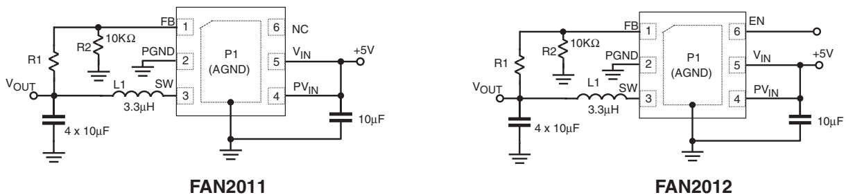
Figure 1. Typical Application
