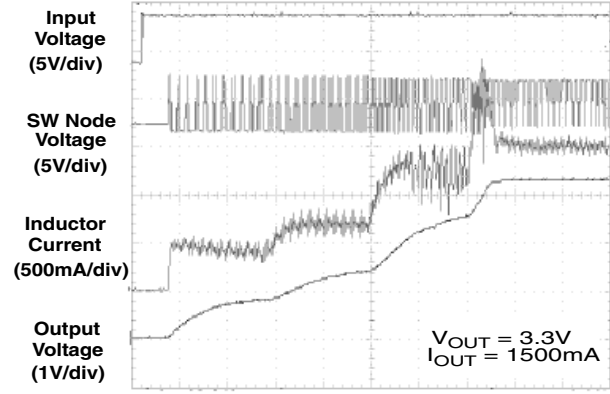
Start-up Response
