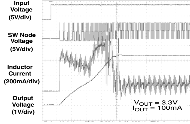
Start-up Response
