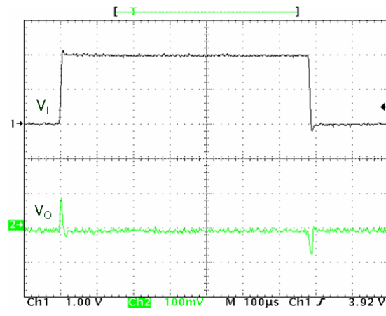
Figure 18. Line transient
