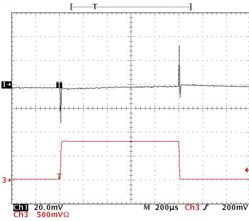
Figure 17. Load transient
