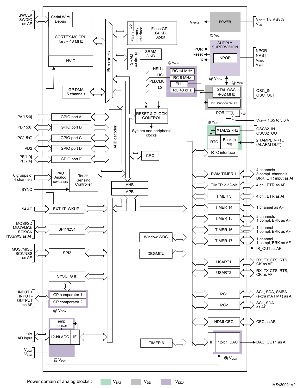
Figure 1. Block diagram
