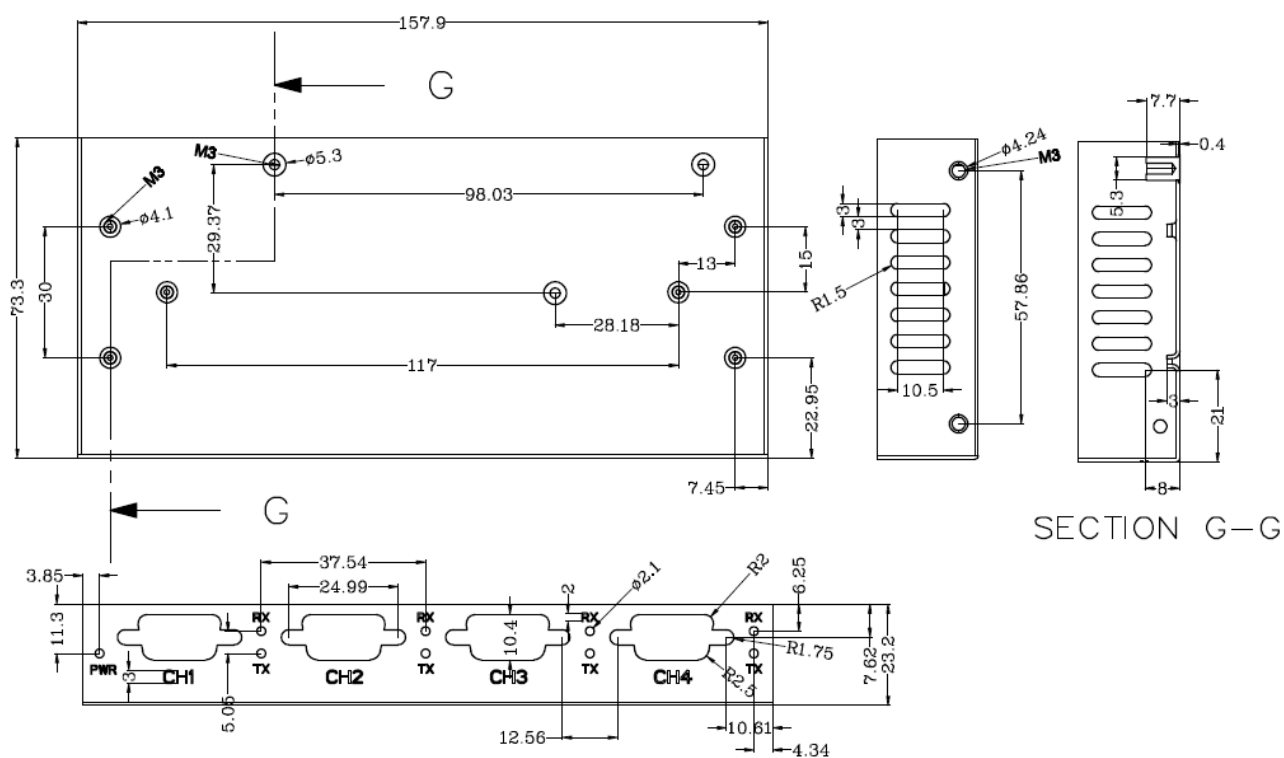
Figure 5.6 - USB2-H-1004-M Bottom Cover Dimensions
