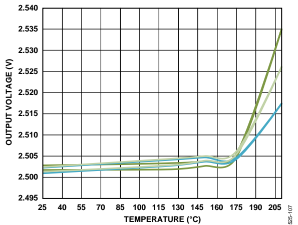
Figure 19. Thermal Hysteresis, I_{LOAD} = 0\text{ mA} , FLATPACK Package
