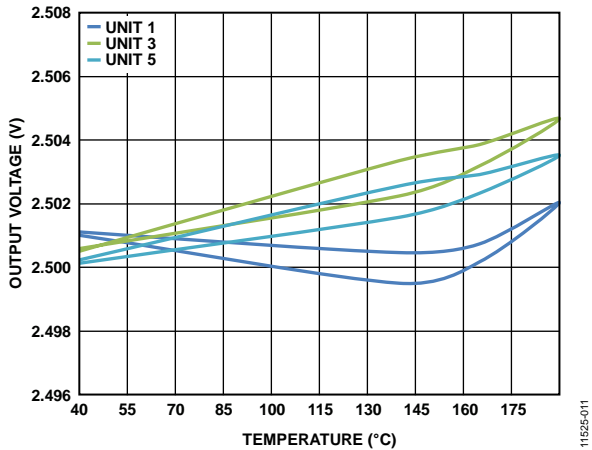
Figure 16. Thermal Hysteresis, I_{LOAD} = 0\text{ mA}
