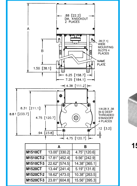
Motor-Driven Single, Two and Three-Ganged, Cased
