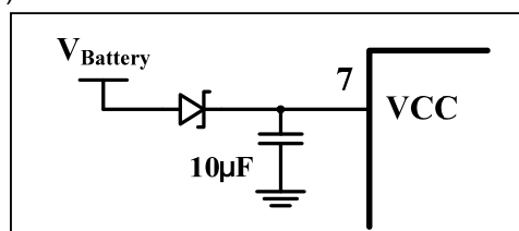
Figure 23 Capacitor For Latch Status
