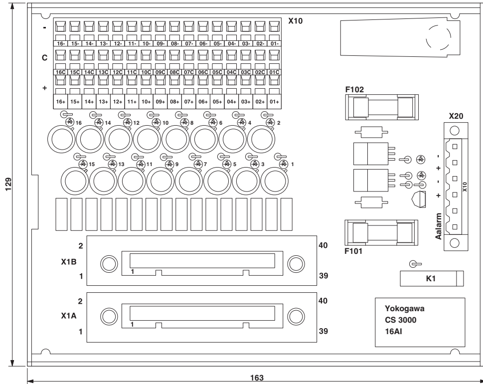
Dimensional drawing
