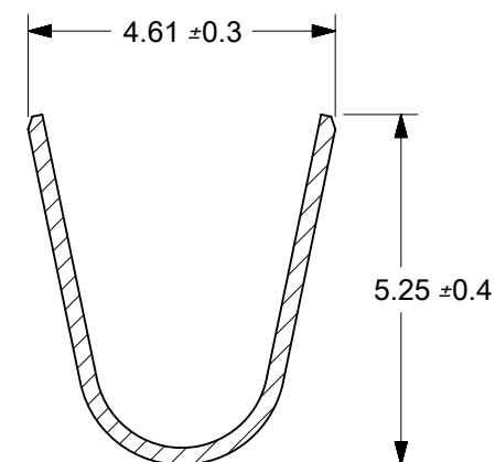
SECTION Y-Y
