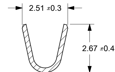
SECTION Z-Z
