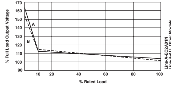
Typical Load Regulation
