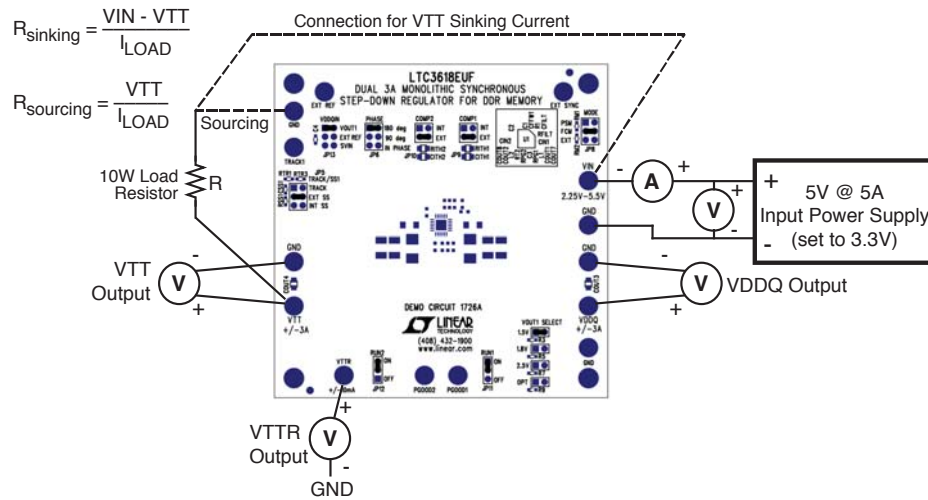
Figure 2. Proper Measurement Equipment Setup
