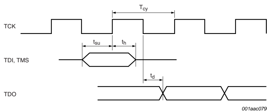
Fig 35. Boundary scan timing diagram
