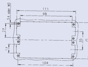
Panel cut out (insert)
