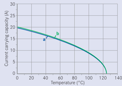
Curve a: 1.5 mm² wire gauge
