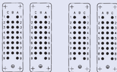
Stamped contacts
