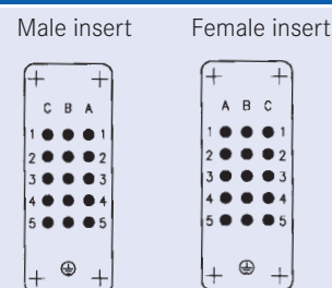
Stamped contacts
