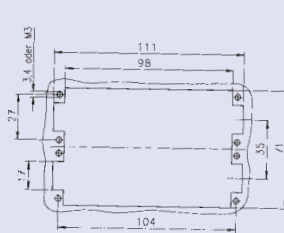
Panel cut out (insert)
