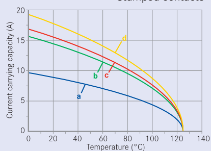
Stamped contacts
