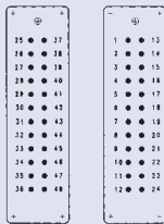
Female insert
