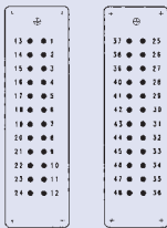
Male insert
