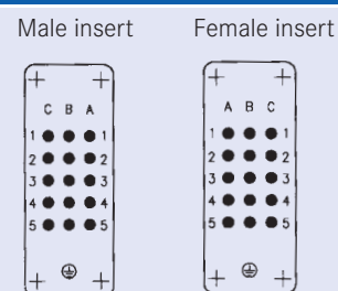
Stamped contacts
