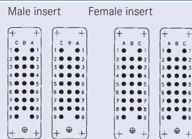
Stamped contacts
