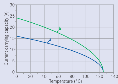
Curve b: 2.5 mm² wire gauge
